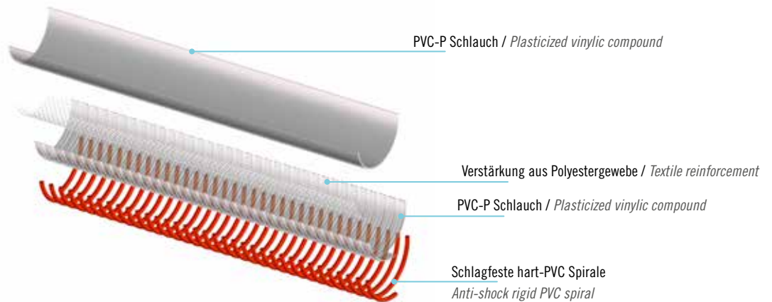
Spiralina verfügbar (Cod. SC WT) Banding coil available (Code SC WT)
